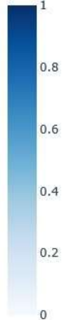
Cosine Similarity
