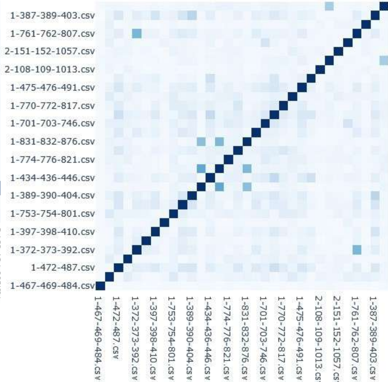
Cosine Similarity
